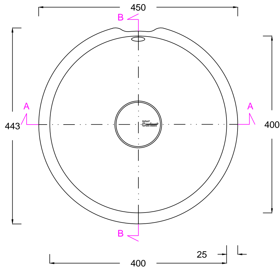
PLAN VIEW
